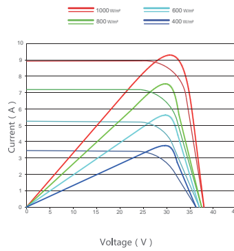
Current-Voltage & Power-Voltage Curves (260W)
